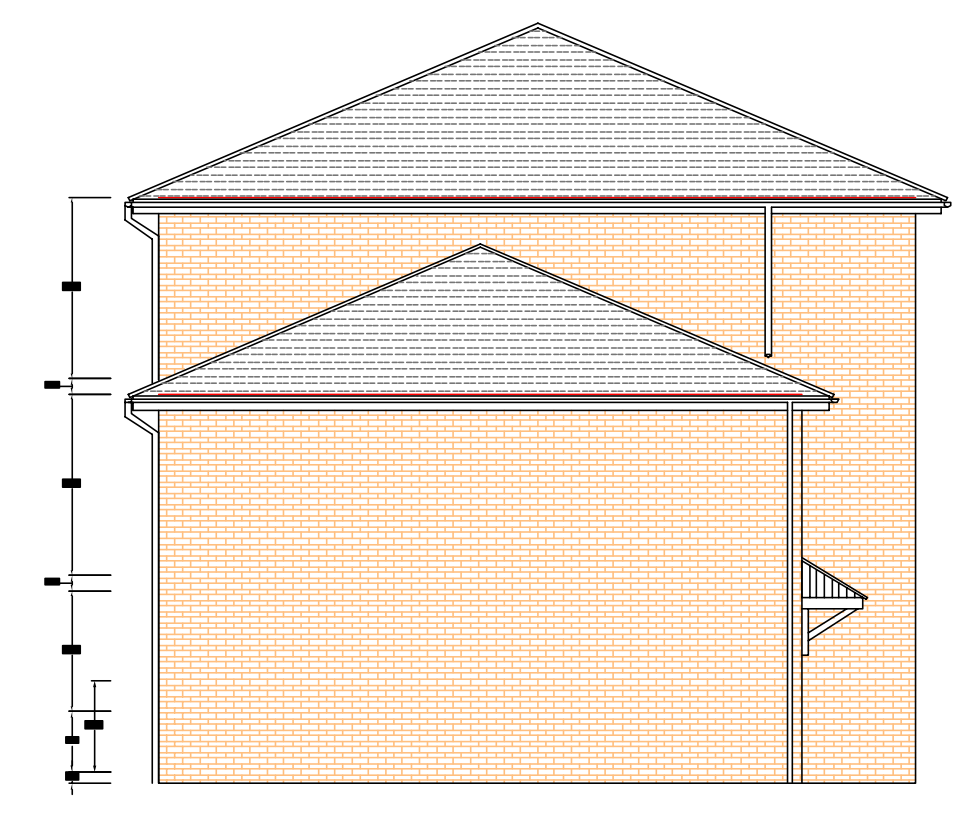
SIDE ELEVATION - VIEW B
