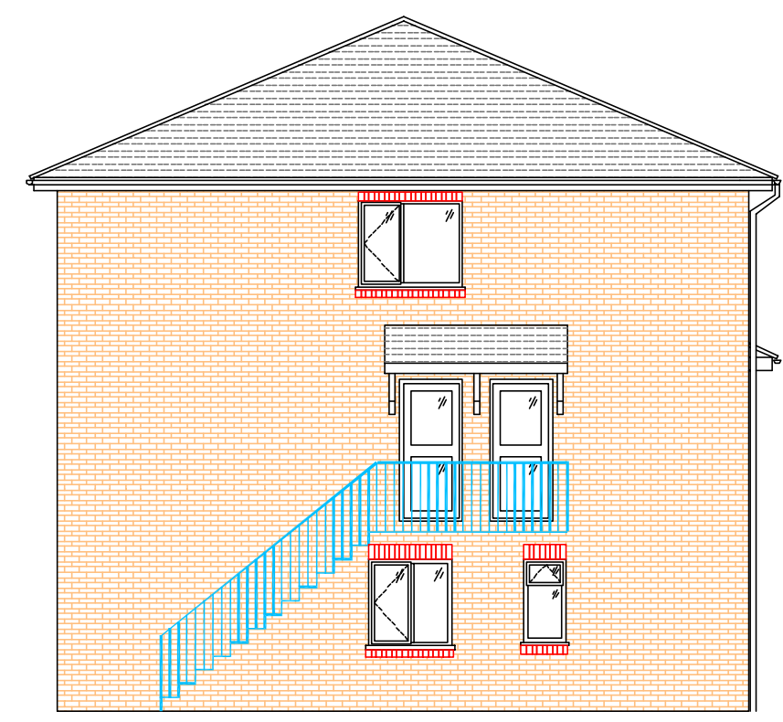
REAR ELEVATION - VIEW D
